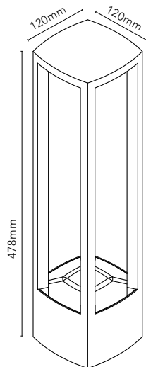
MIRAGE OUTDOOR STAND
