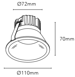
CURVE II Ø110
