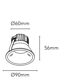
CURVE II Ø90
