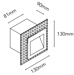
DELI 1 mounting box (Included)
